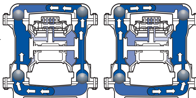
Right chamber—discharge Left chamber—suction
