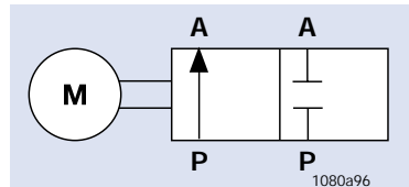
3/2 Way Valve Connection B + R Closed
