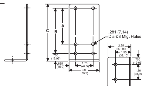
Fig. 3 Side Mount Bracket
