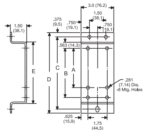
Fig. 3 Side Mount Bracket
