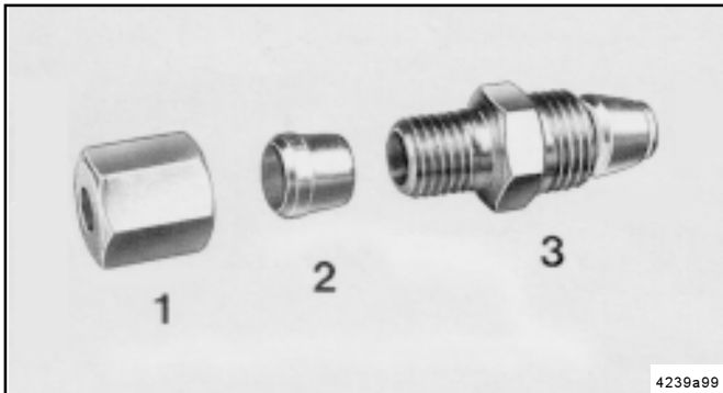
Fig. 24 - Single parts of the check valve
