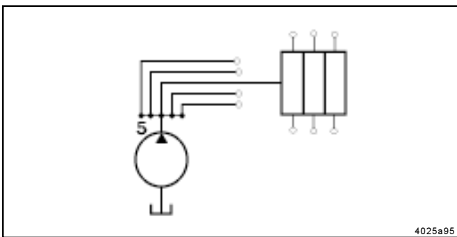
Fig. 7 - Multiline pump expanded by a progressive metering device
