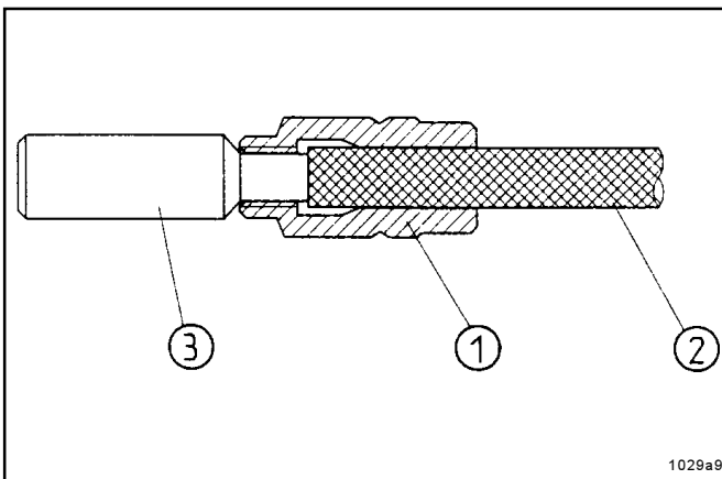
Fig. 31 - Preassembly of the threaded sleeve by means of an adjusting gauge
