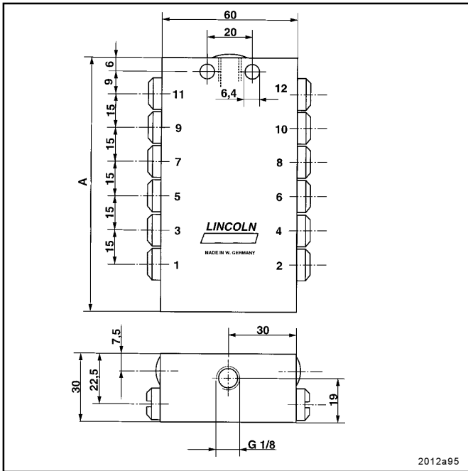
Metering Devices Model SSV 6 to SSV 22 (Blocks)
