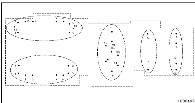
Fig. 35 - Combining the lubrication points into groups
