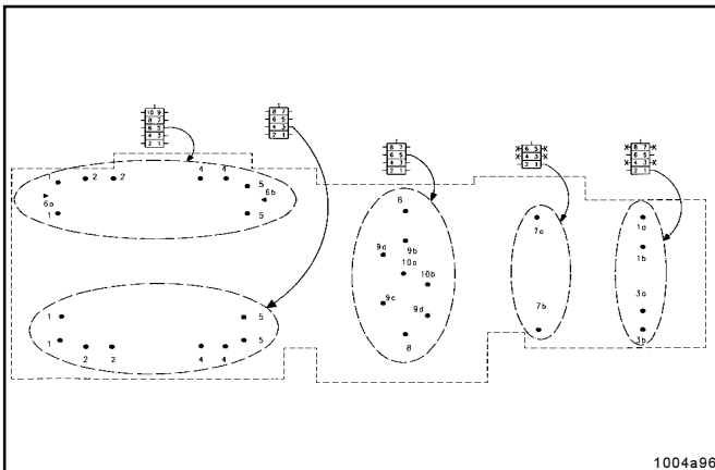
Fig. 37 - Allocating the metering devices
