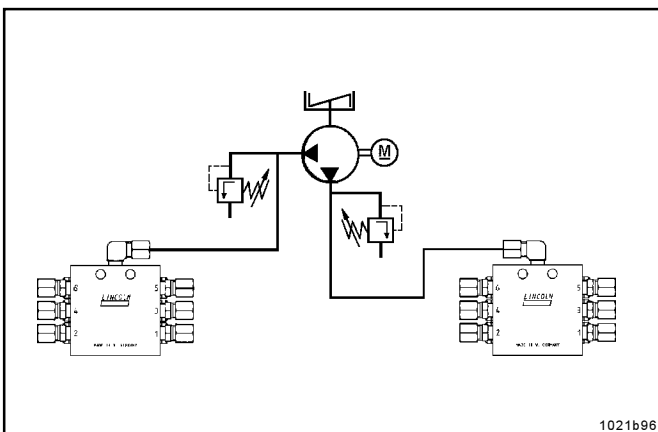
Fig. 47 - System using two pump elements
