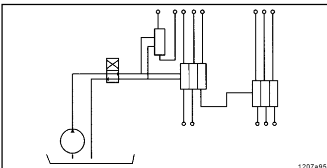
Fig. 8 - Two-line system expanded by a progressive metering device
