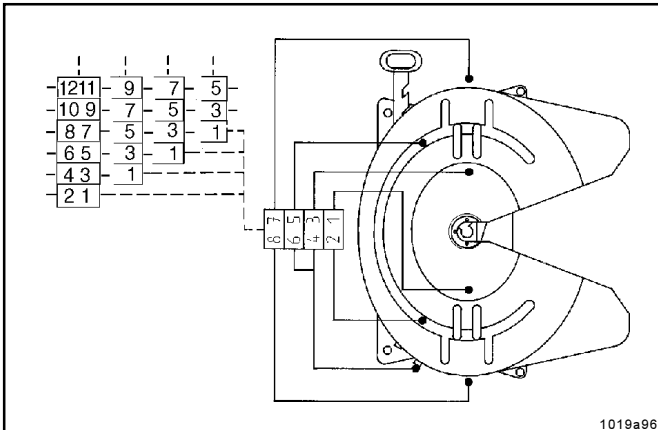
Fig. 45 - Fifth-wheel with 7 lubrication points
