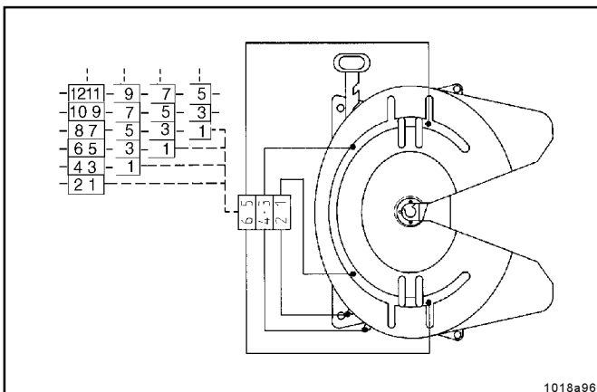
Fig. 44 - Fifth-wheel with 6 lubrication points
