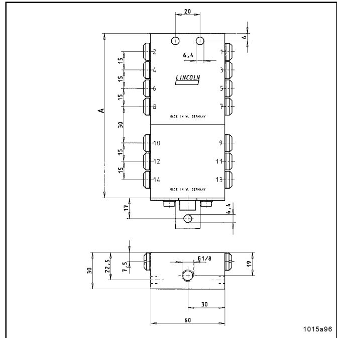
Metering devices SSV 14 ... 22 (assembled)
