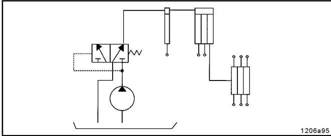
Fig. 9 - Single-line system expanded by a progressive metering device
