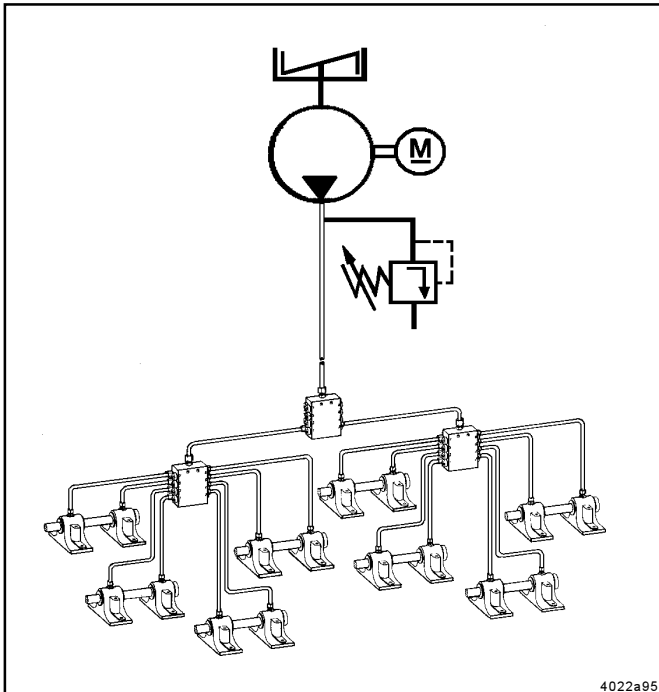
Fig. 43 - Example of connection for machine bearings
