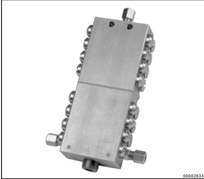
Fig. 23 - Lubricant metering device, assembled model SSV 16
