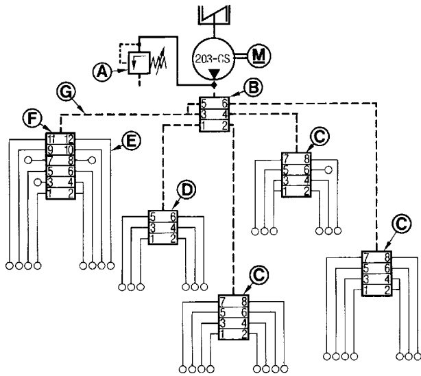
Fig. 32 - Example of a lubrication system
