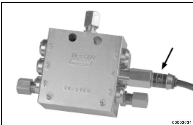
Fig. 17 - Piston detector installed on the metering device
