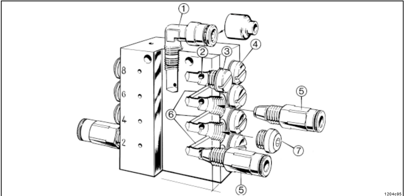
Fig. 21 - Install the push-in type outlets fittings and closure plugs in accordance with the dosage
