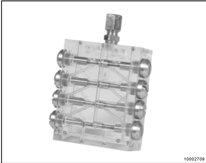
Fig. 2 - Metering device type SSV 8 shown as a demonstration model
