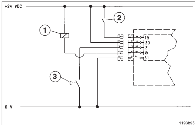
Fig. 7 - Connection diagram
