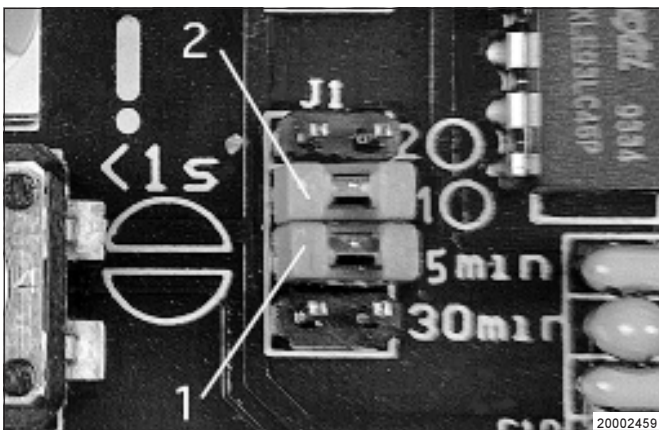
Fig. 10- Monitoring ranges
