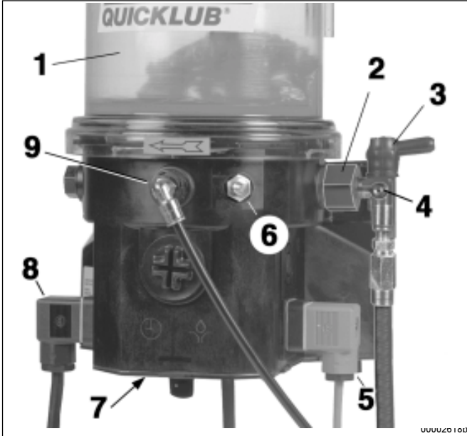
Fig. 2 - Pump components
