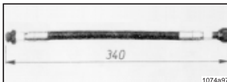
Extension hose Part-No. 251-14043-1
