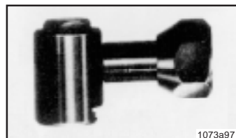
Connecting tube with pull coupler Lubrication fitting DIA 16 Part-No. 251-14043-6 Lubrication fitting DIA 22 Part-No. 251-14043-8
