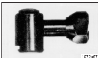
Connecting tube with push coupler Lubrication fitting DIA 16 Part-No. 251-14043-6 Lubrication fitting DIA 22 Part-No. 251-14043-8
