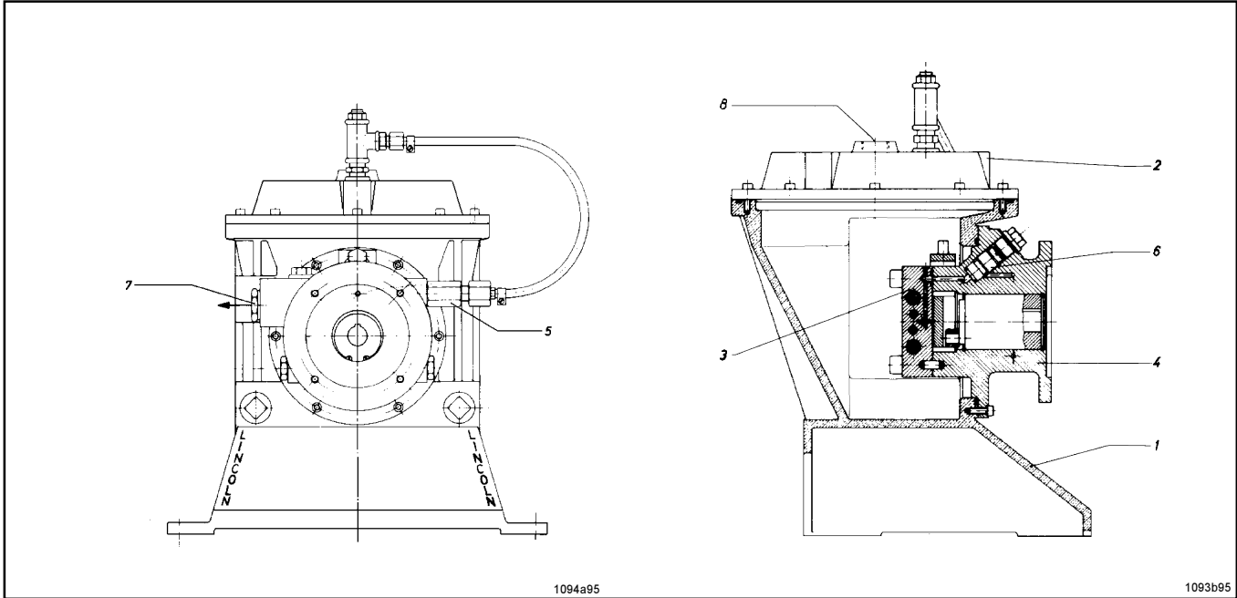
Fig. 2.4.1: Sectional drawing of pump ZPU09 ZPU 09
