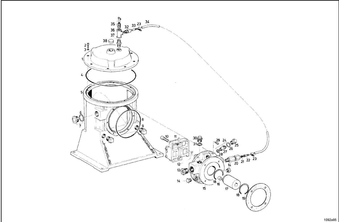
Abb 5.1.1: High-Pressure Central Lubrication pump ZPU 09
