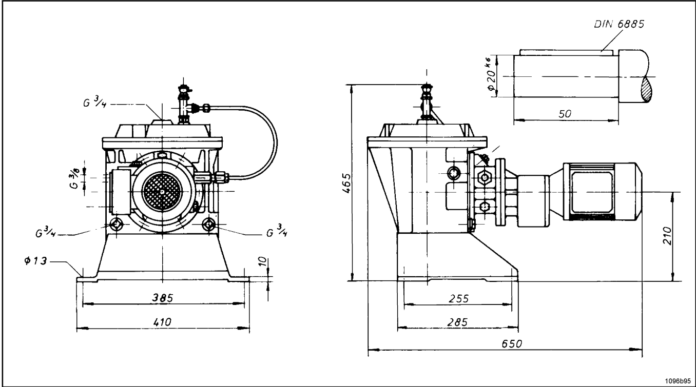
Fig. 6.2.1: Dimensional Drawing ZPU09
