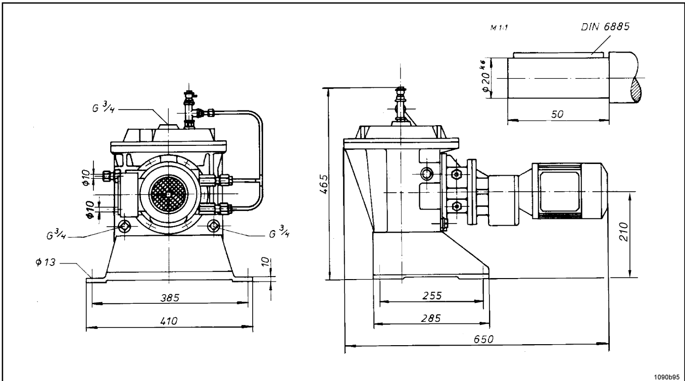
Fig. 6.2.1: Dimensional Drawing ZPU09A
