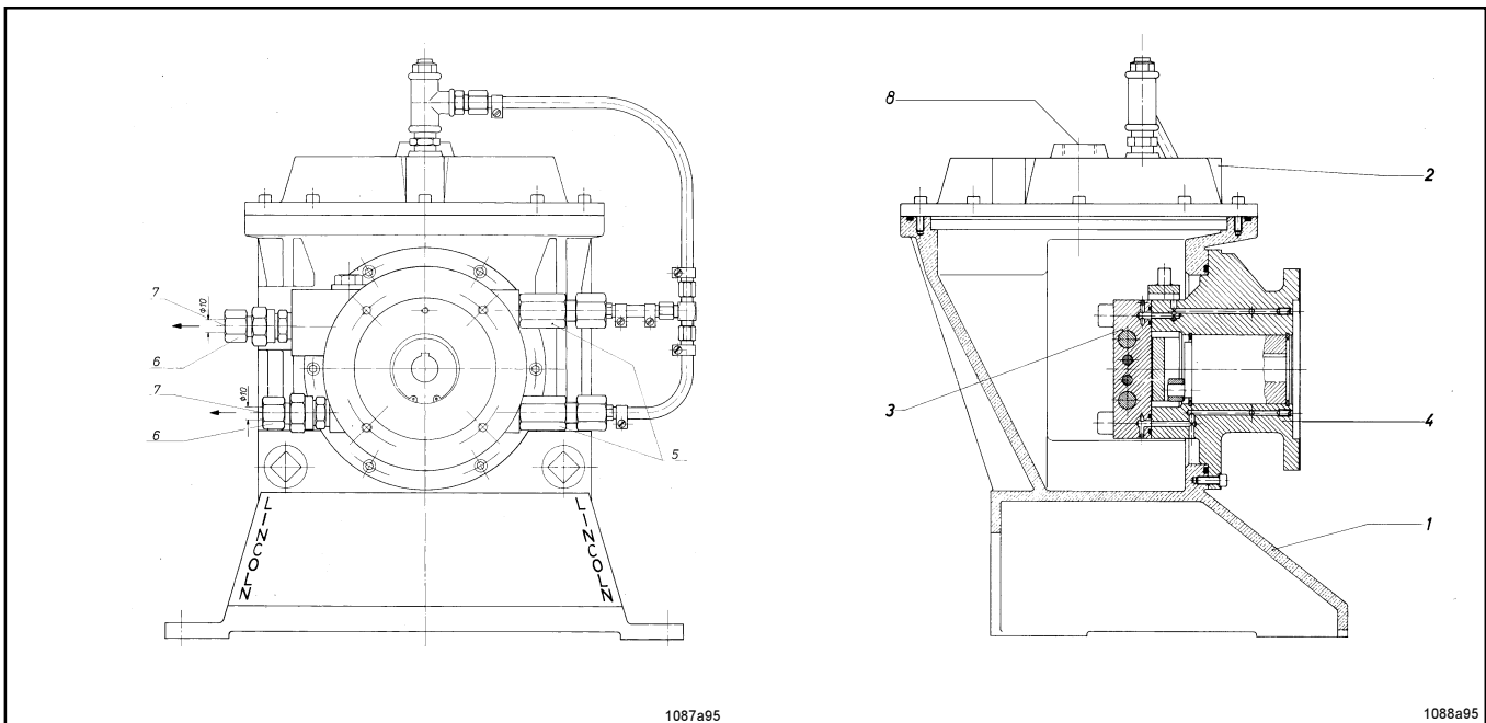
Fig. 2.4.2: Sectional drawing of pump ZPU09A
