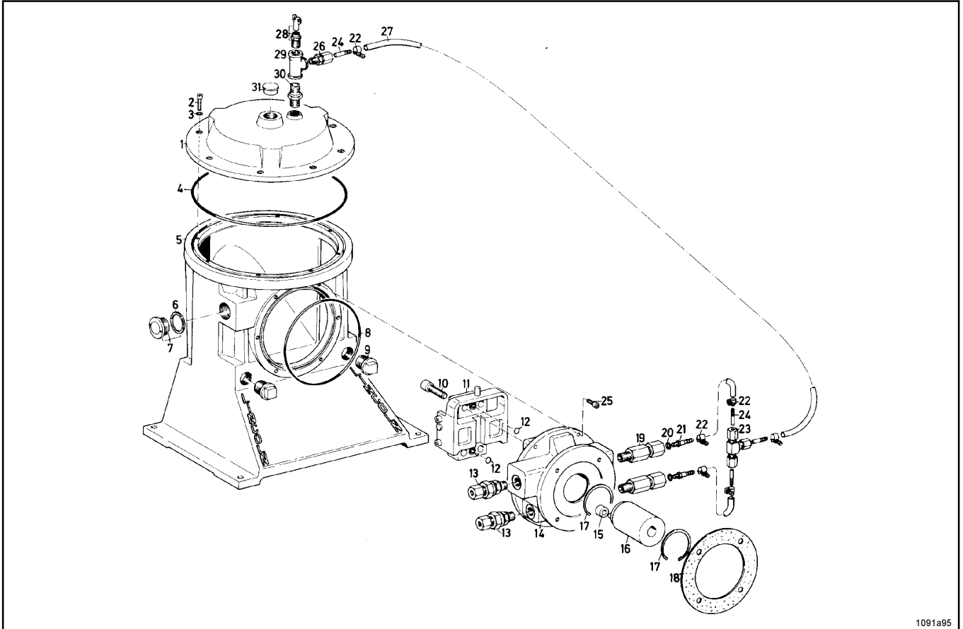
Fig.5.2.1: High-Pressure Central Lubrication pump ZPU 09A
