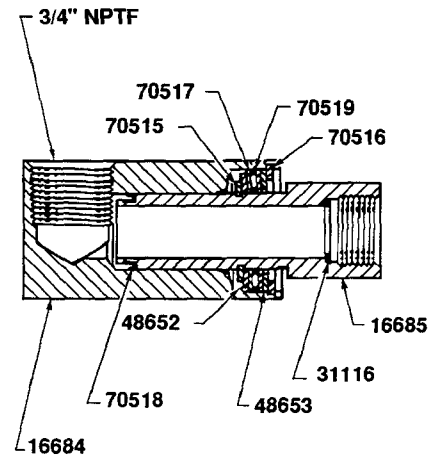
84679 SWIVEL ASSEMBLY
