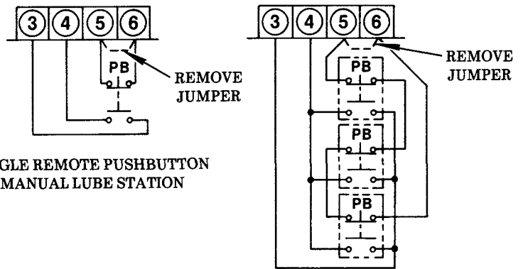
MULTIPLE REMOTE PUSHBUTTONS MANUAL LUBE STATIONS
