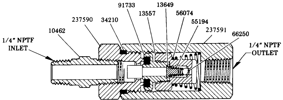
83114 CHECK ASSEMBLY
