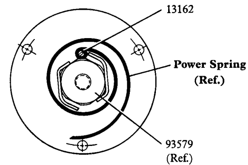
SPRING POSITION
