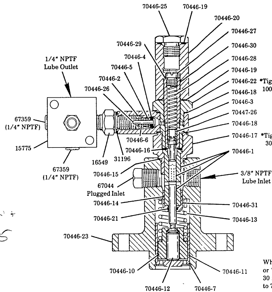
MODEL 130305 7MM PUMP HEAD ASSEMBLY
