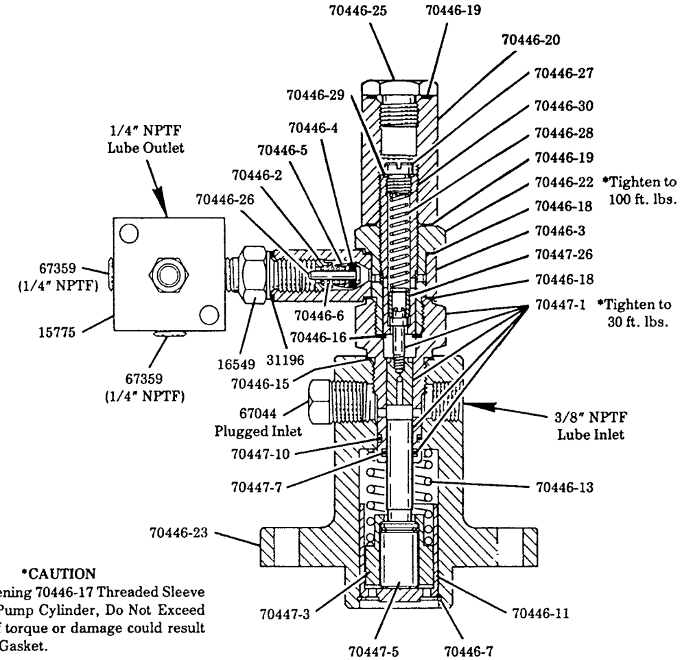
MODEL 130306 11MM PUMP HEAD ASSEMBLY
